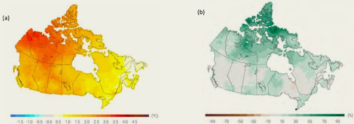
Canadian change in annual average (a) temperature from 1948 to 2016 [ \sim 1.7 °C nationwide] (b) precipitation from 1948 to 2012 [ \sim 20\% nationwide]. Temperature is projected to increase from one to several degrees (depending on carbon emission levels), and precipitation from 5% to over 20%, before the year 2100. Images are from Canada's Changing Climate Report 2019.
